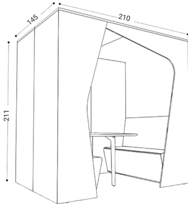
Cabine 4 places
