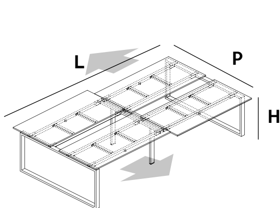
Bench 4 postes
