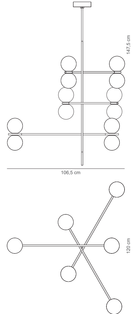
Suspension Grace 2
