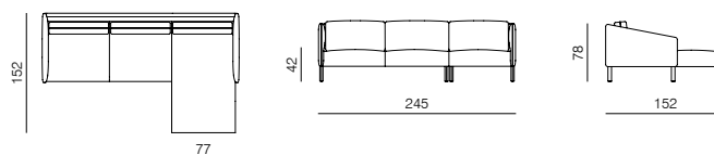
5 2.5SEATER + CHAISE LONGUE w 245 x d 152 x h 78 cm
